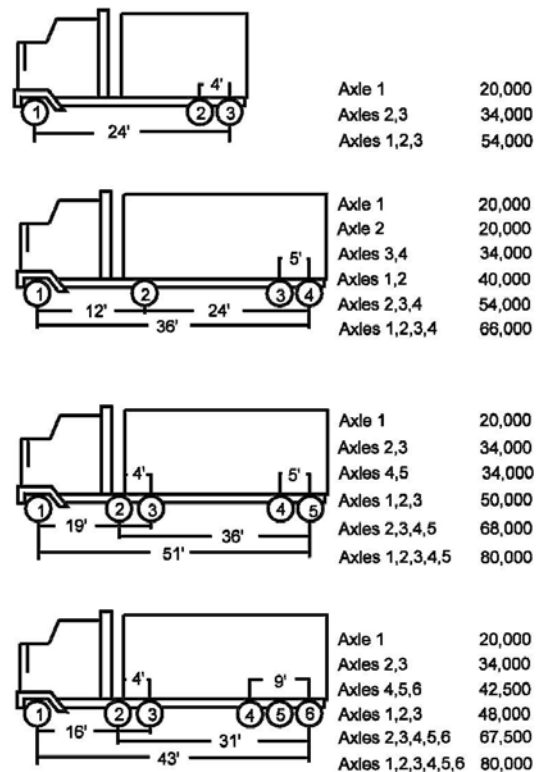
Maximum loading for typical vehicles Vehicle or Combination Maximum Weight - Pounds
